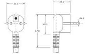
SFS5610/CEE7 Stand VII Class 1 10/16 A 250 V
