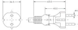
SFS5610/CEE7 Stand IV Class 1 10/16 A 250 V
